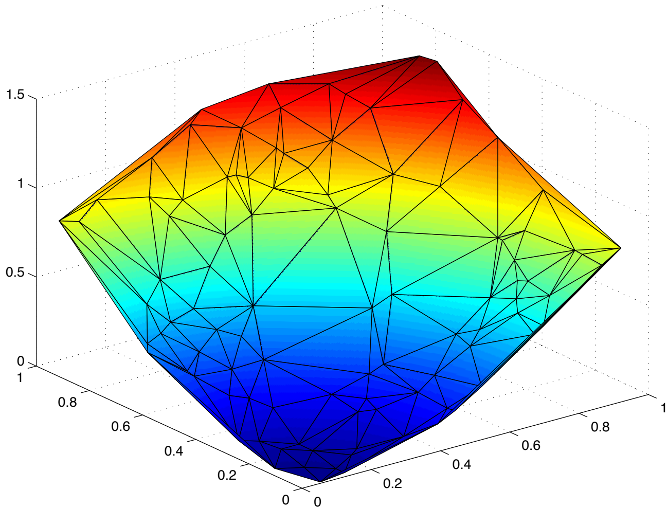
trisurf: example 4
