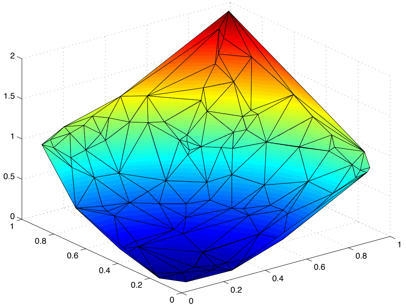
trisurf: example 3
