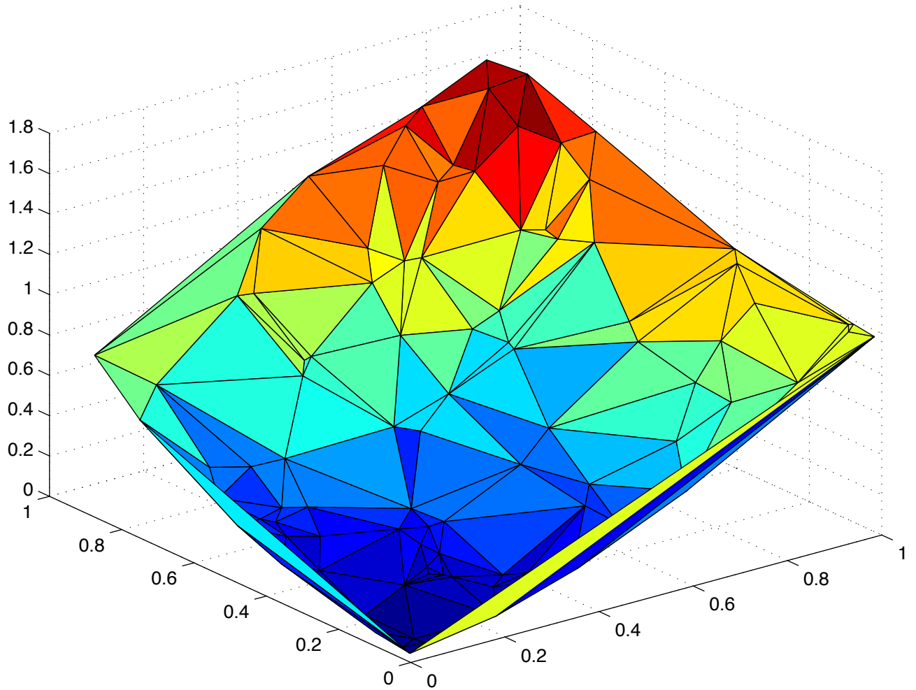
trisurf: example 2
