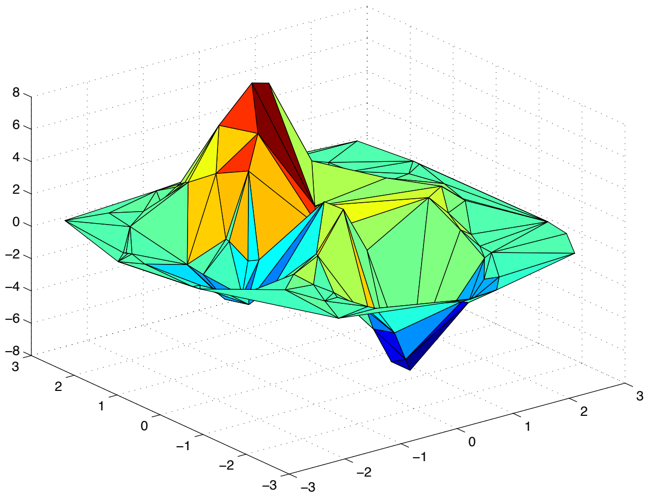
trisurf: example 1
